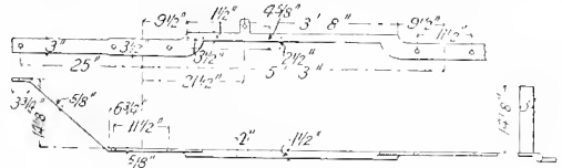
Figs. 5035-37. PEDESTAL TIE-BAR.
